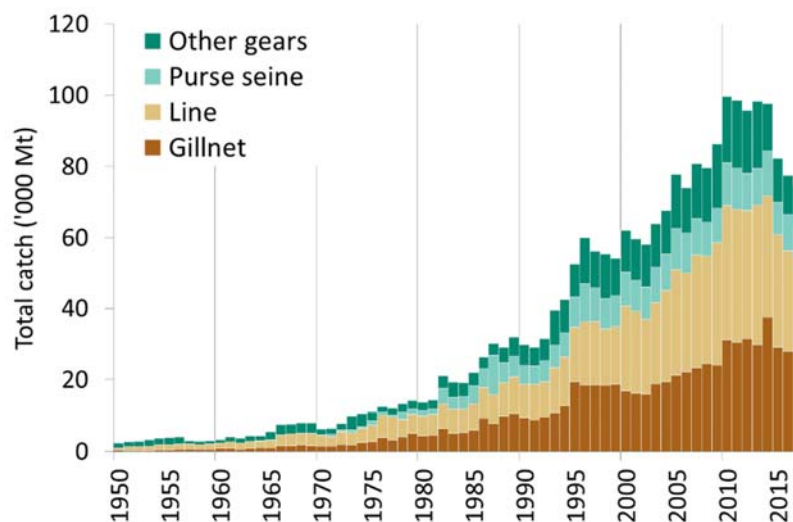
Fig. 1. Frigate tuna: Annual catches of frigate tuna by gear recorded in the IOTC Database (1950–2017) 1 .
