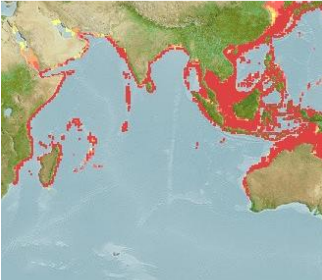
Figure 1. Distribution of T. tonggol in the Indian Ocean 1
